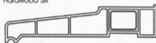
150mm PVCu Sill
